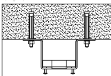
1-CEILING-MOUNT BRACKET
